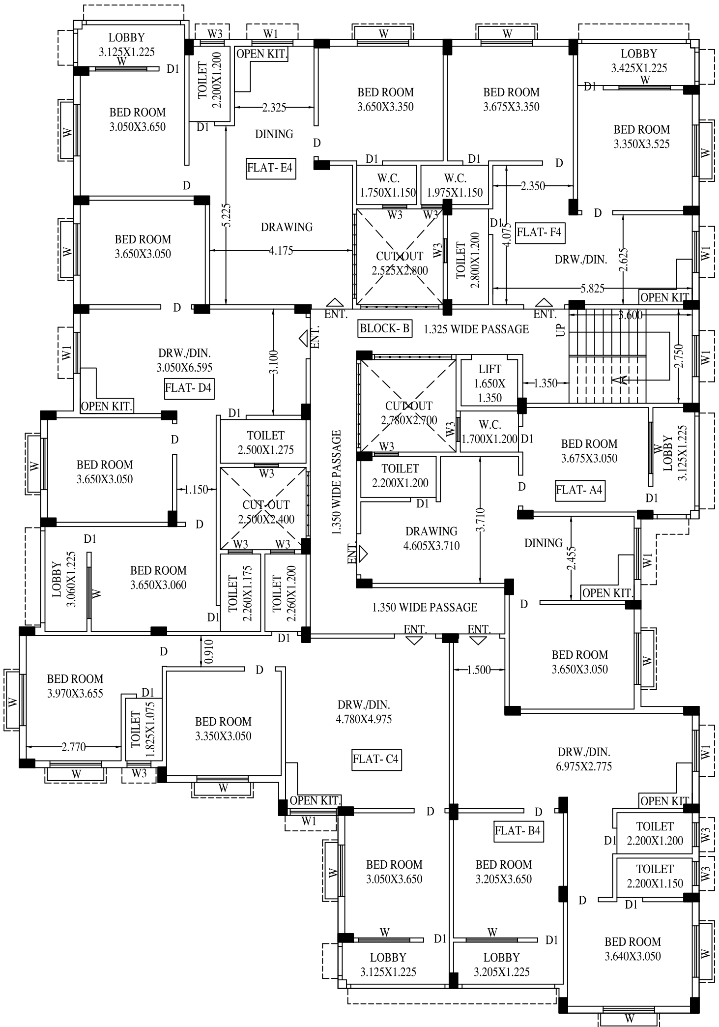
FOURTH FLOOR PLAN SCALE:- 1:100
